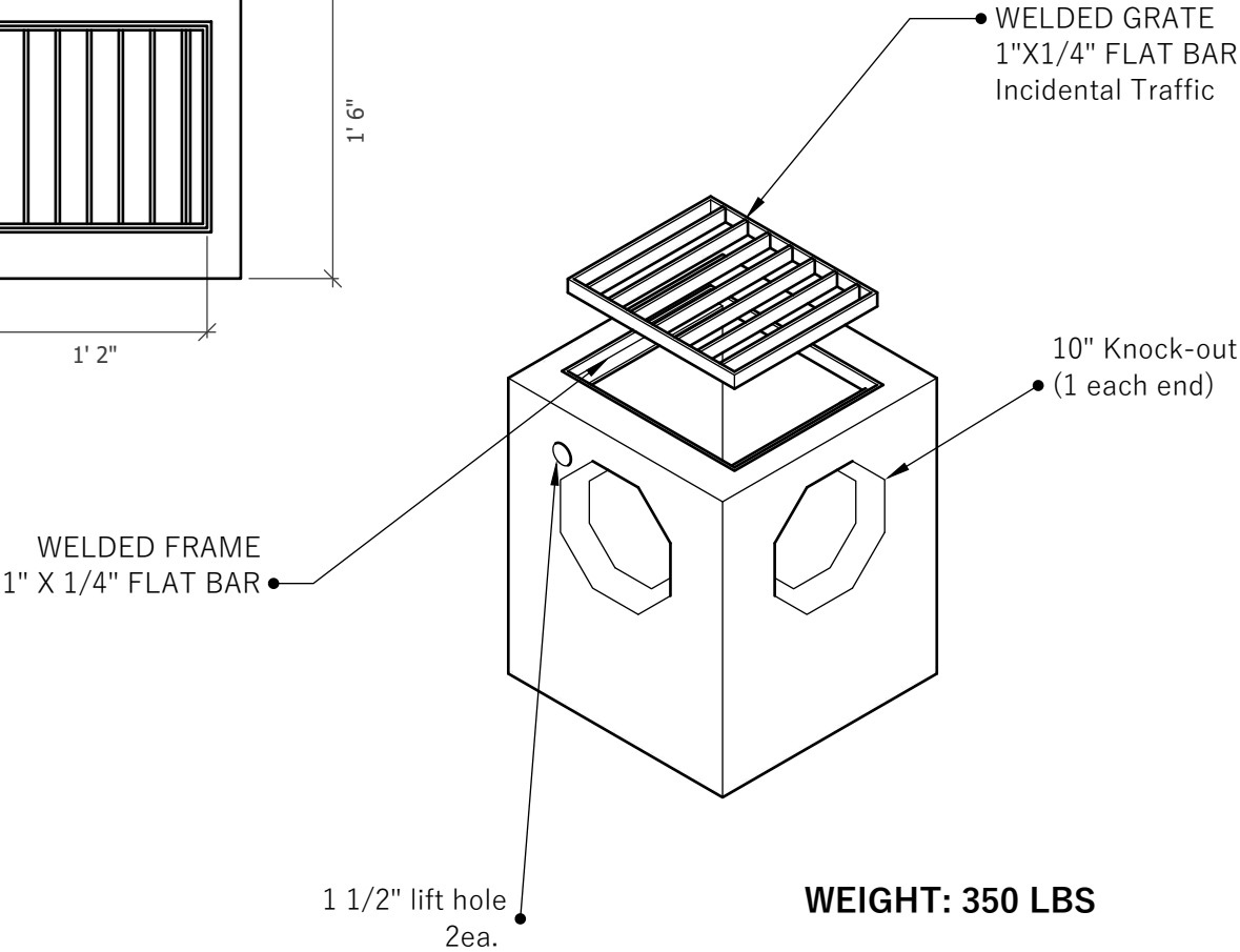
ISOMETRIC
